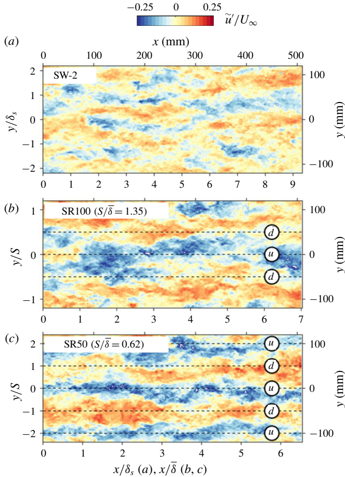
FIGURE 16. Snapshot of \tilde{u} (turbulent fluctuations and mean spanwise variation) for (a) the reference smooth-wall case SW-2, (b) SR100 and (c) SR50, taken from WPIV measurements. Dashed lines are the spanwise locations related to the common flow up (ⓐ) and common flow down (ⓓ) of the mean secondary flows.
